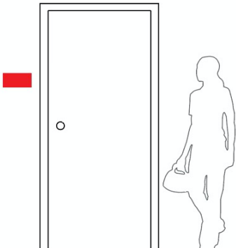
2 ELEVATION - SINGLE DOOR NTS
